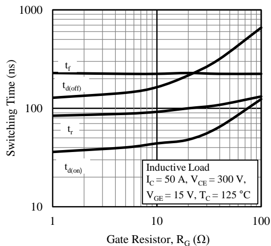
Figure 14. Switching Time vs. Gate Resistor
