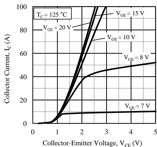
Figure 6. Output Characteristics ( T_C = 125 °C)
