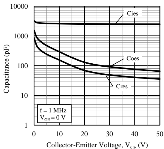
Figure 11. Capacitance Characteristics
