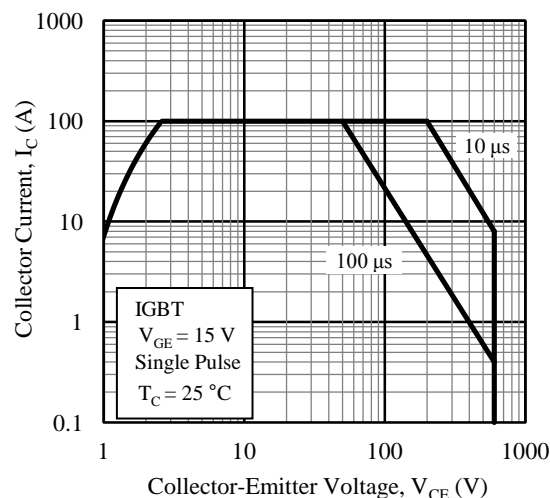
Figure 2. Safe Operating Area
